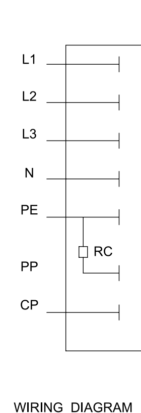
WIRING DIAGRAM
