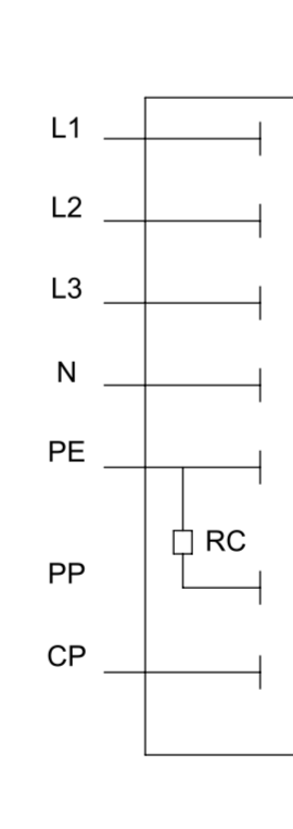
WIRING DIAGRAM
