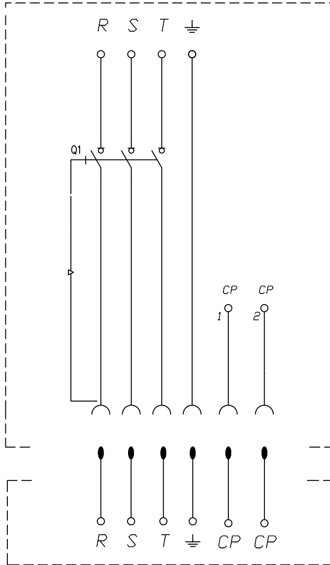
PLUG
